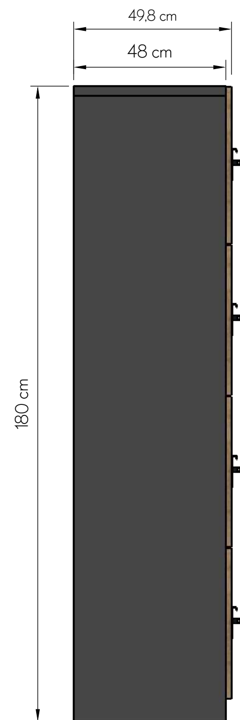
SIDE VIEW
