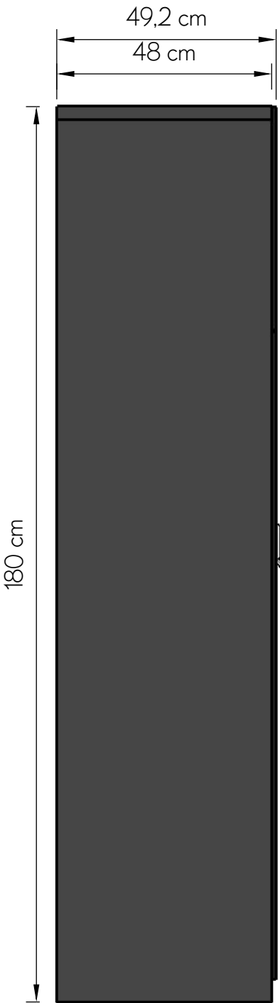
SIDE VIEW
