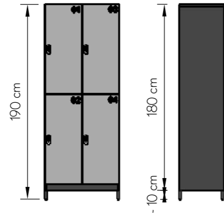
LOCKER ON ADJUSTABLE LEGS
