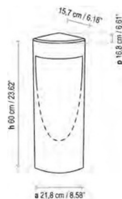
Moai B/60 IP66
