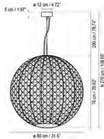
Nans Sphere PF/80 IP-66
