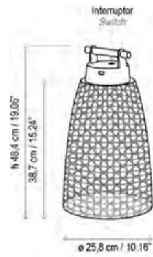
Nans Portable M/49/R IP-65
