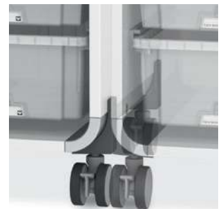
Magnetic linking system for connecting several caddies, e.g. to form a material cabinet
